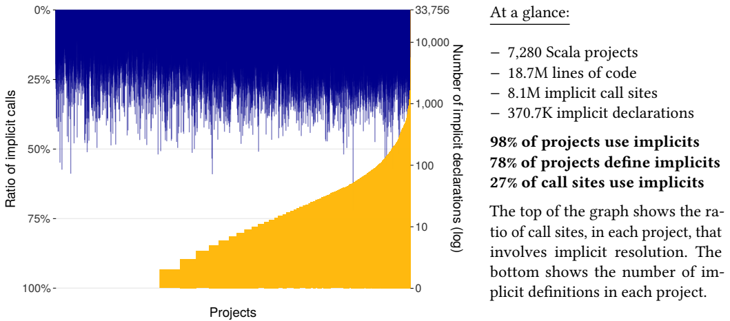
Fig. 1. Implicits usage across our corpus
