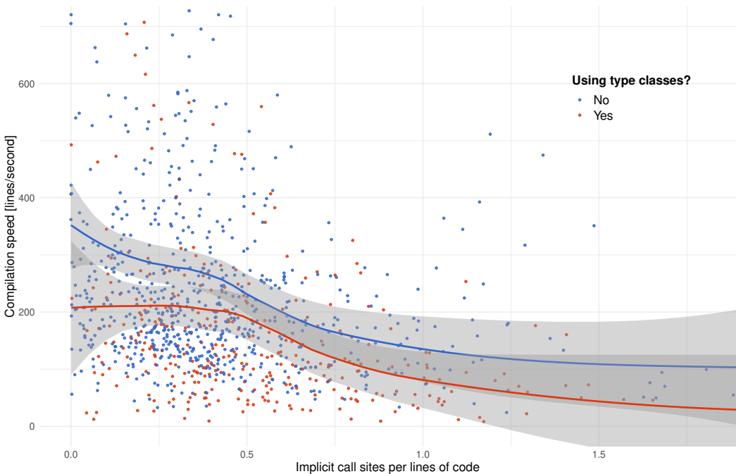
Fig. 11. Compilation slowdown
