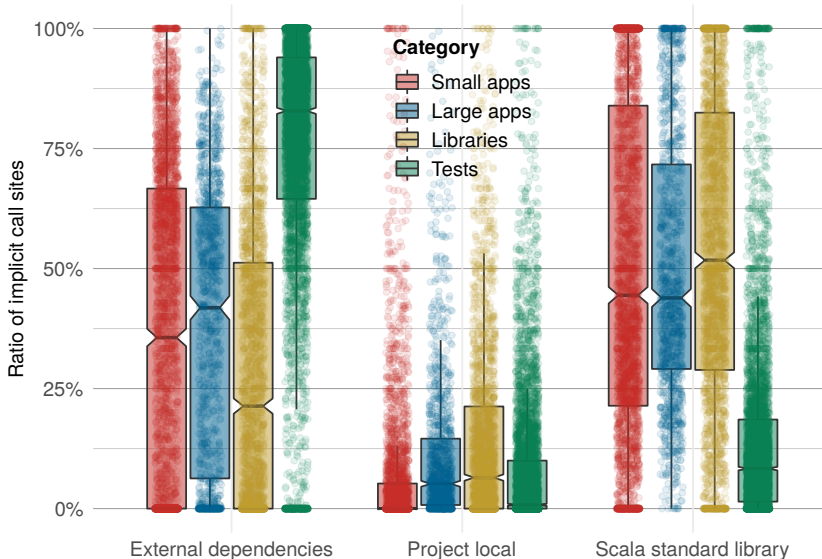
Fig. 8. Origin of parameter declarations
